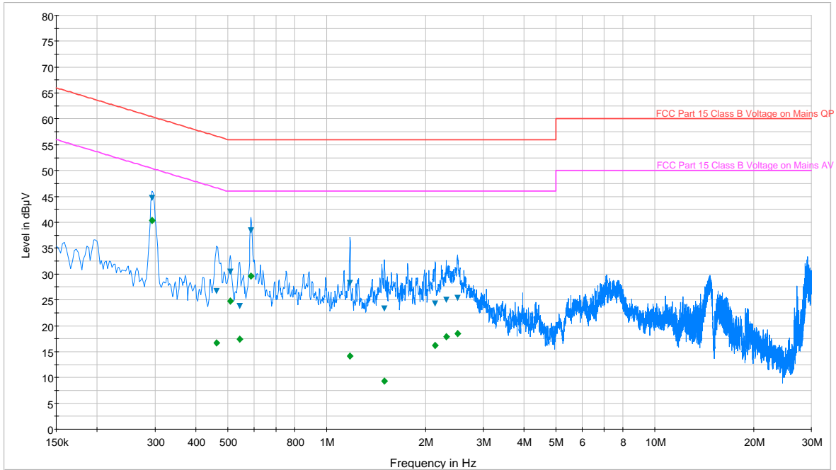
Plot 6-15. Line Conducted Mains Plot with Bluetooth LE (L1)
