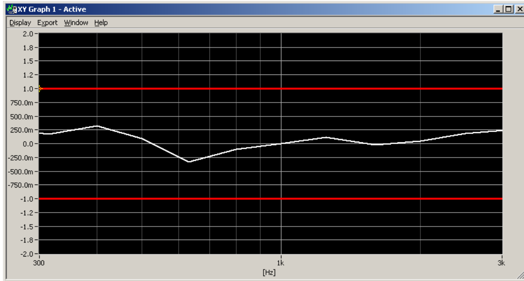
Figure 7-3 Helmholtz Coil Validation for Frequency Response
