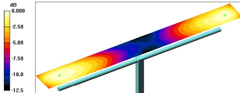
0 dB = 164.7V/m
