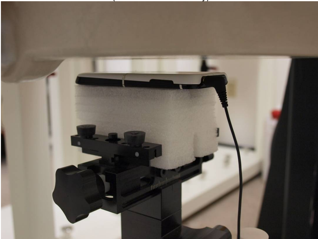
Body-hotspot: Rear w/ 10 mm separation distance with Headset (for WCDMA mode only)
