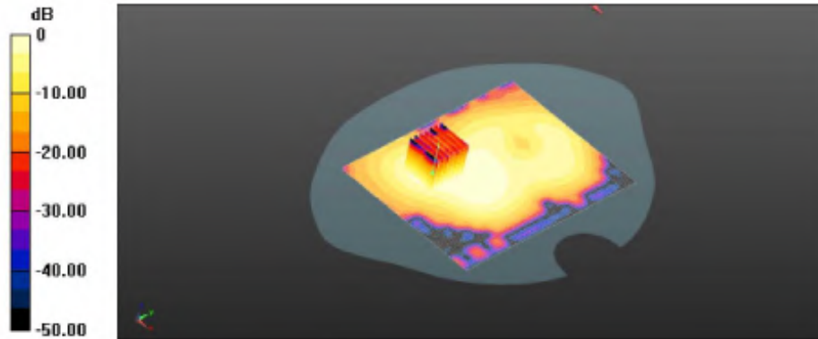
0 dB = 0.123 W/kg = -9.10 dBW/kg
