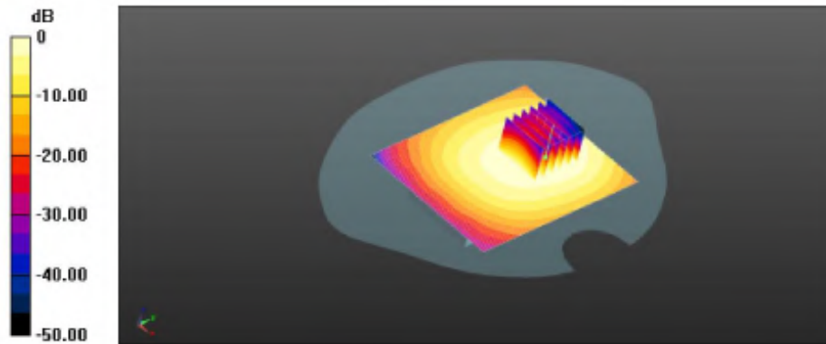
0 dB = 0.750 W/kg = -1.25 dBW/kg
