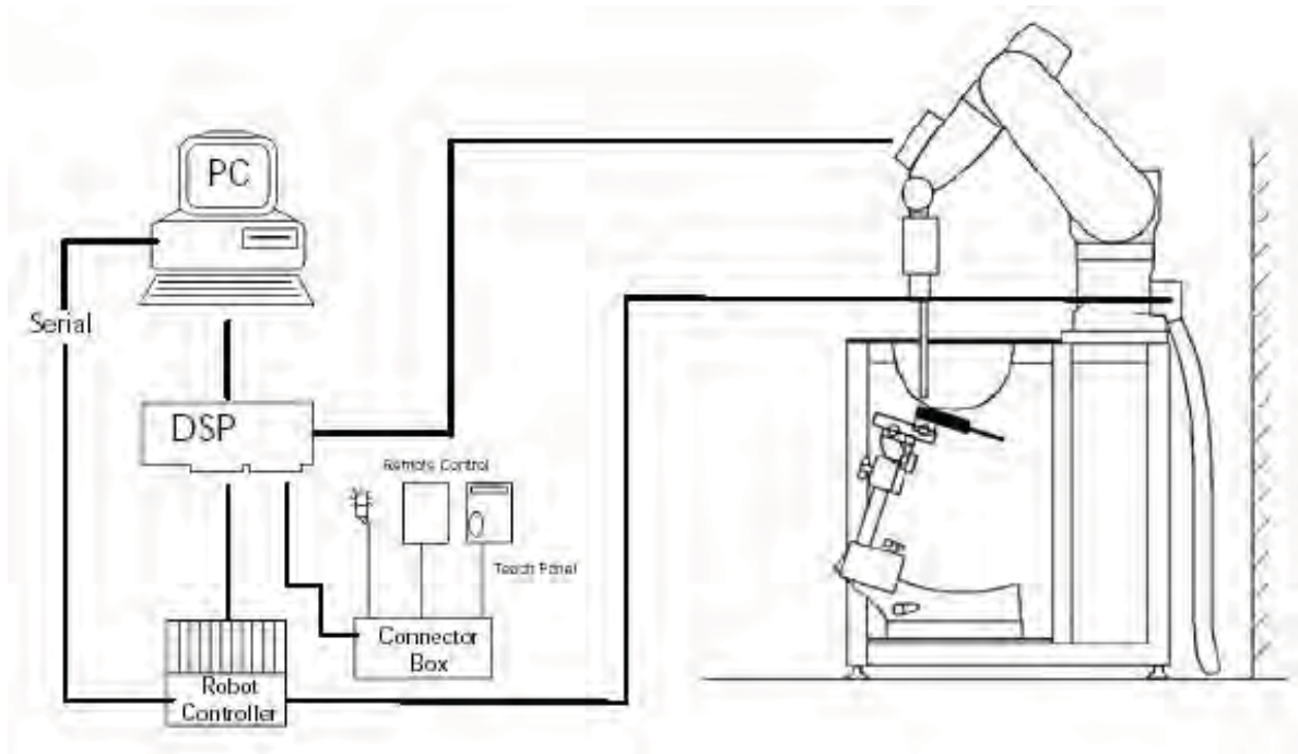
Figure 3.1 SAR Measurement System Setup
