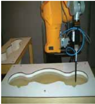
Figure 3.8 SimulatedTissue
