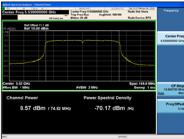
802.11ac_VHT80 UNII 2C BAND Average Power (5530MHz) CH 106MCS0
