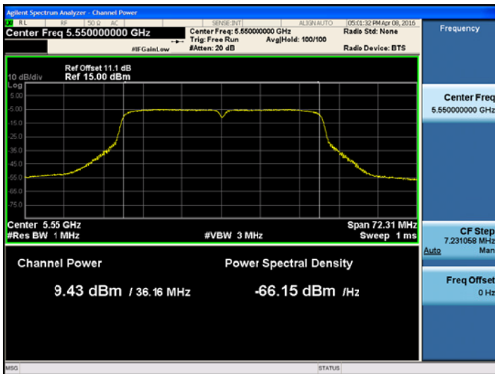
802.11n_HT40 UNII 2C BAND Average Power (5510 MHz ~5710 MHz) CH 110MCS1
