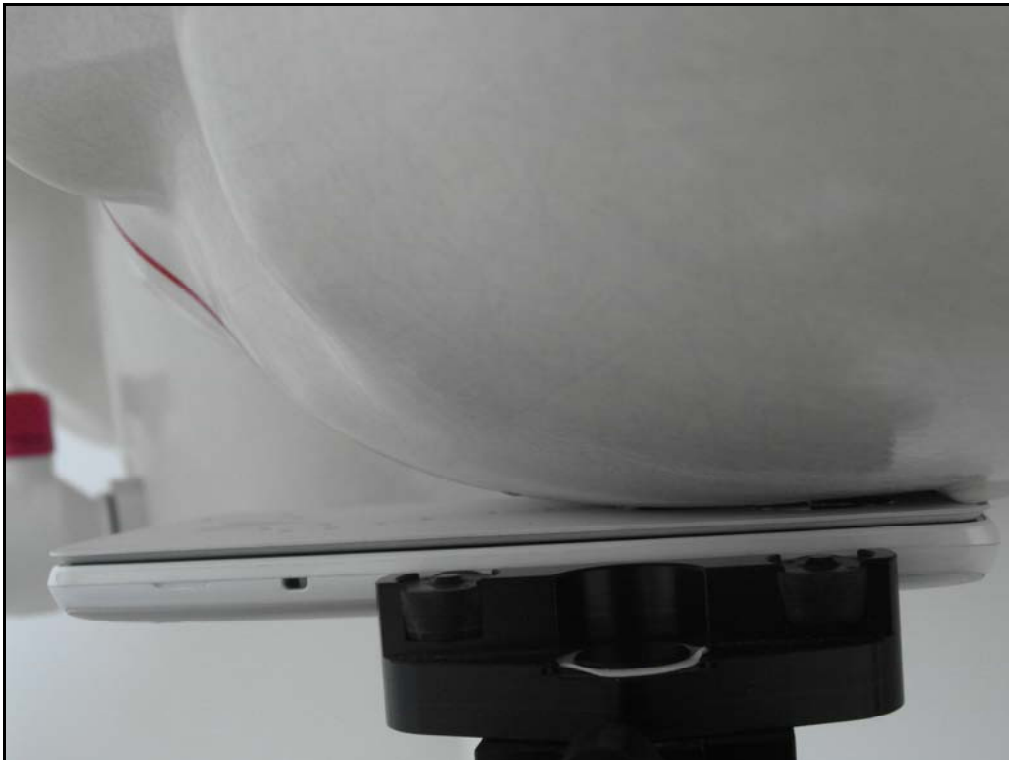
Worst Case Test Head Left Touch with Quick Cover Accessory
