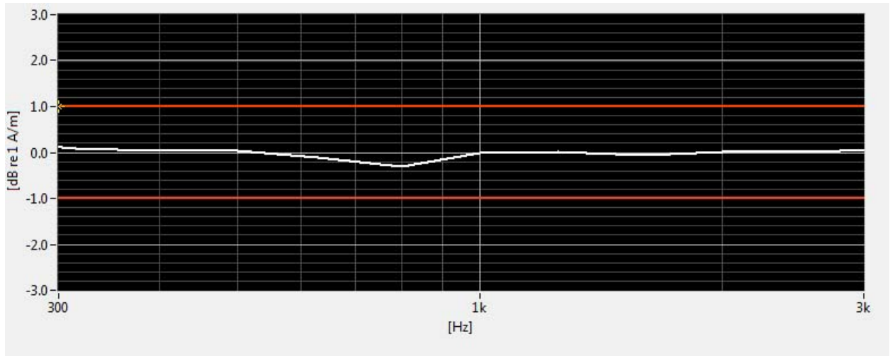
Figure 7-3 Helmholtz Coil Validation for Frequency Response
