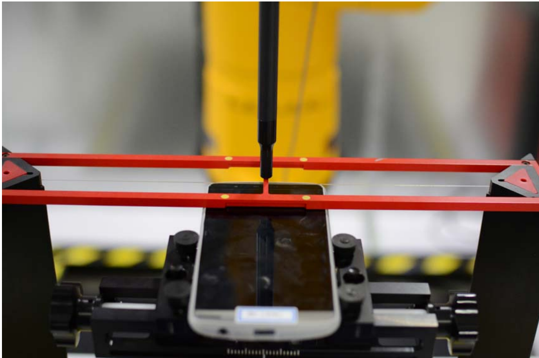
Figure 18-4 Ear Reference Point HAC Phantom Alignment (Wireless Charging Cover)
