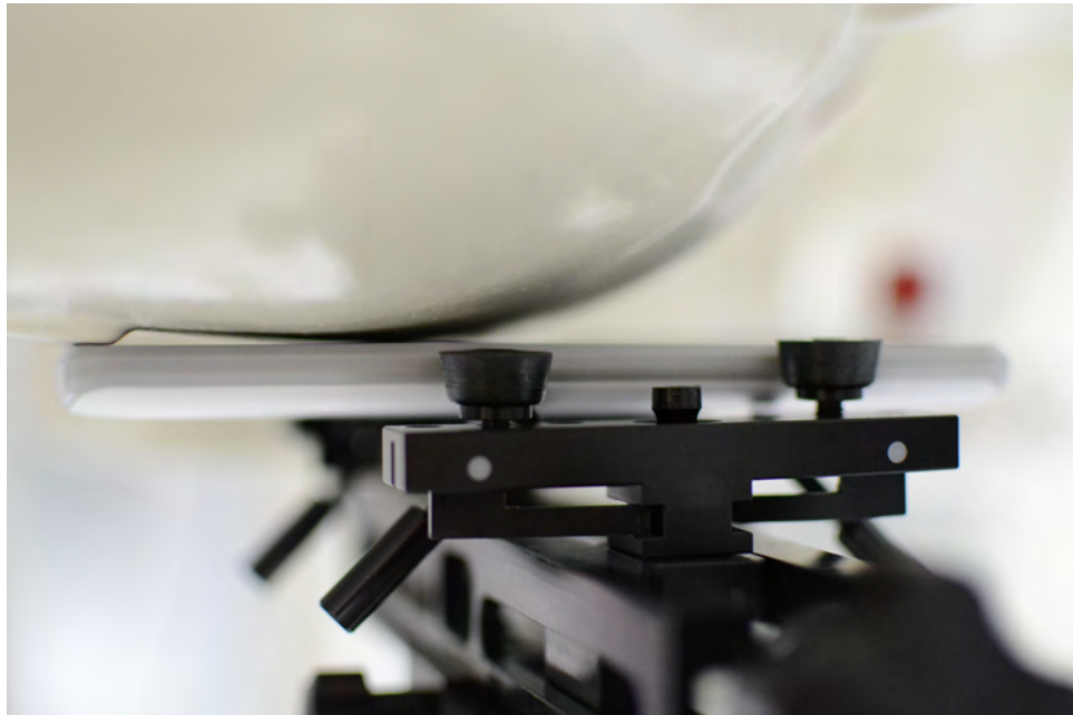
SAR Test Setup Photo 4: Right Cheek with Wireless Charging Back Cover
