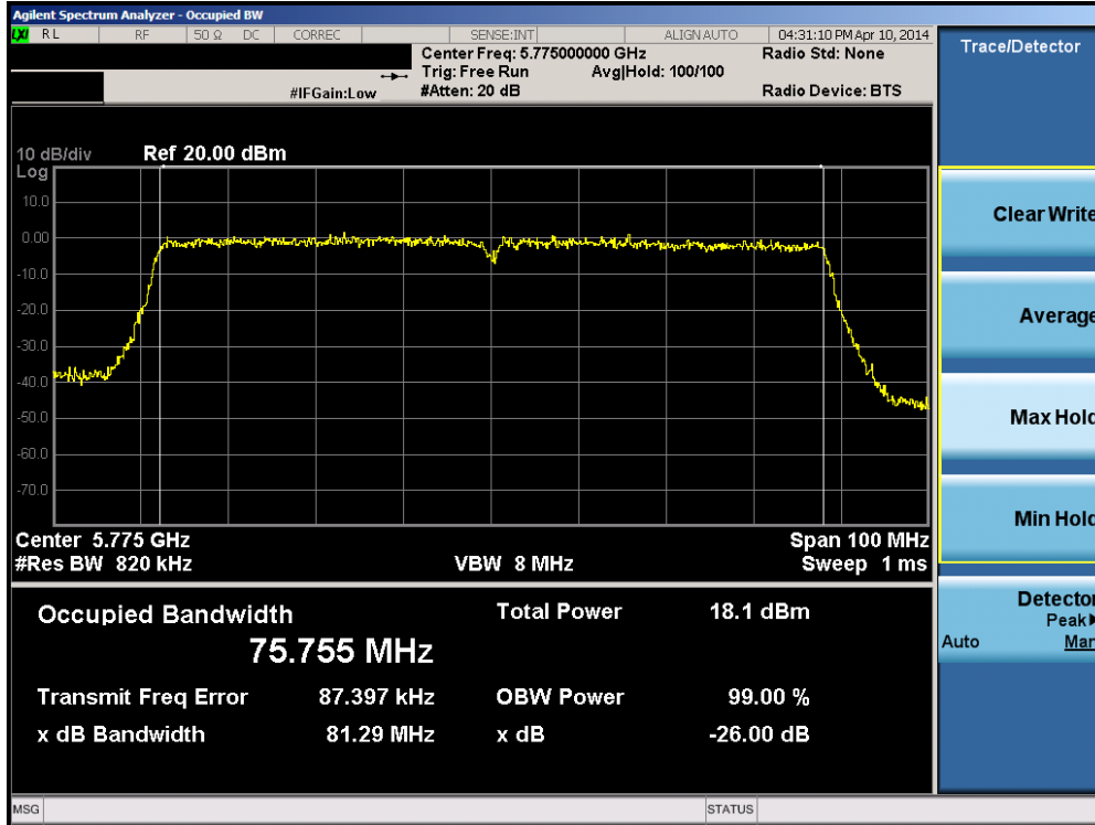
Plot 6-37. 26dB Bandwidth Plot (80MHz BW 802.11ac (UNII Band 3) – Ch. 155)
