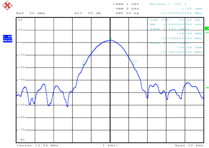
20 dB / 99% Bandwidth Plot on 13.56 MHz
