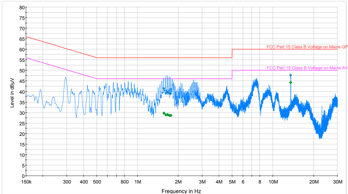
Plot 8-2. Line-Conducted Test Plot (N)
