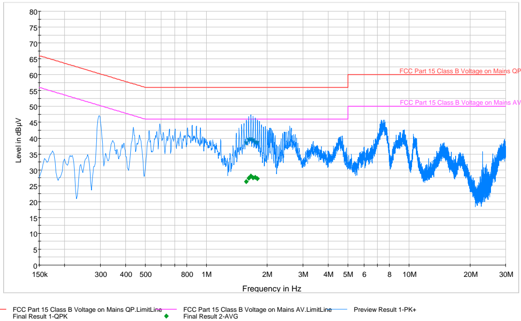
Plot 6-108. Line Conducted Plot with 802.11a UNII Band 2 (N)
