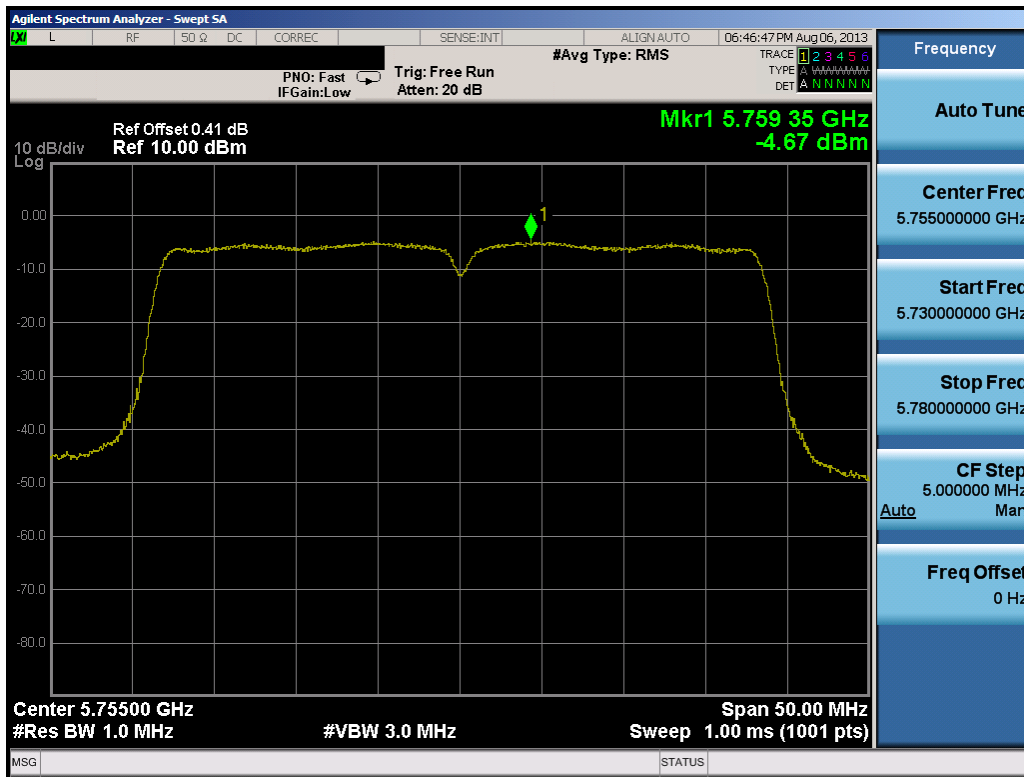
Plot 6-77. Peak Power Spectral Density Plot (40MHz BW 802.11n (UNII Band 4) – Ch. 151)
