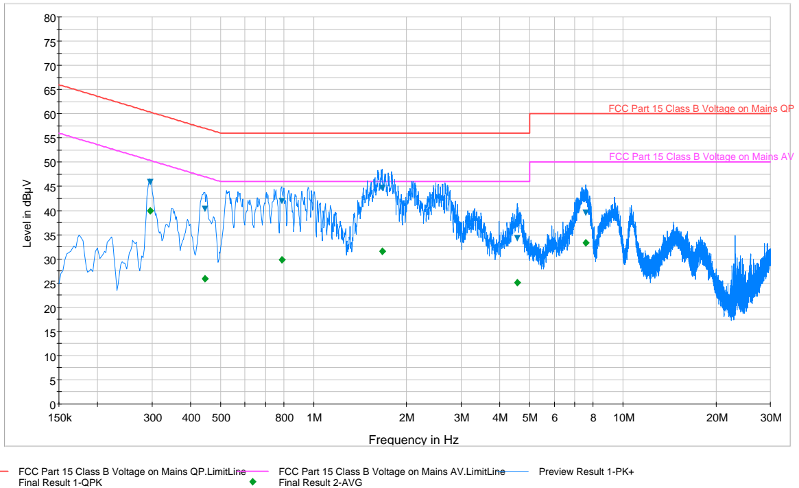
Plot 6-109. Line Conducted Plot with 802.11a UNII Band 3 (L1)
