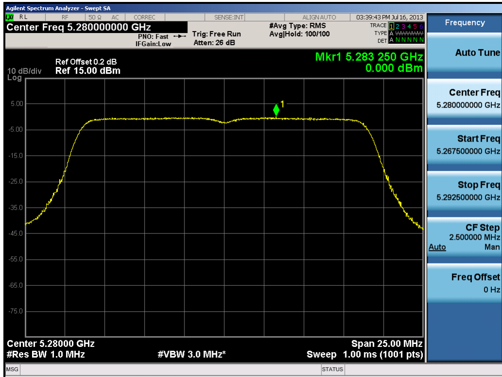
Plot 6-55. Peak Power Spectral Density Plot (20MHz BW 802.11n (UNII Band 2) – Ch. 56)
