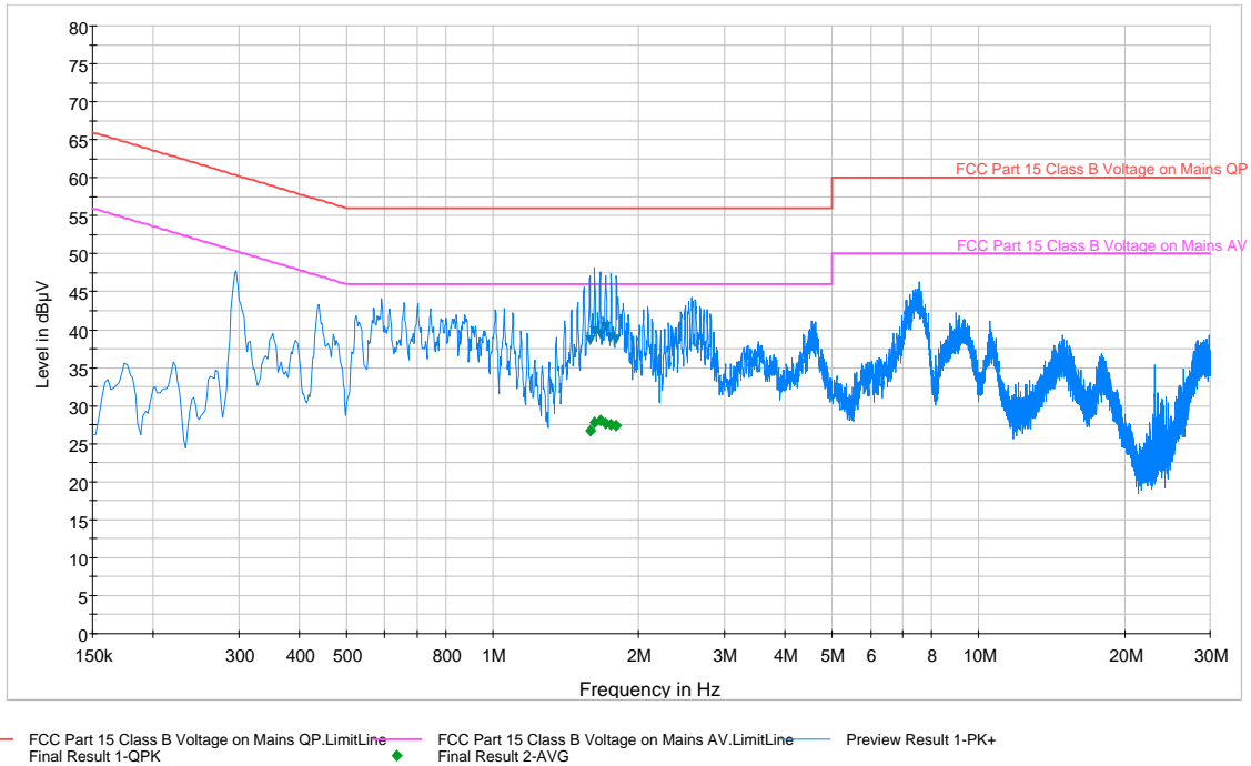
Plot 6-110. Line Conducted Plot with 802.11a UNII Band 3 (N)
