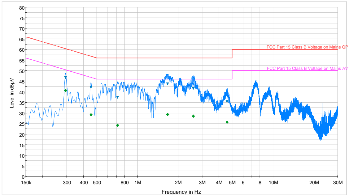
Plot 6-111. Line Conducted Plot with 802.11a UNII Band 4 (L1)
