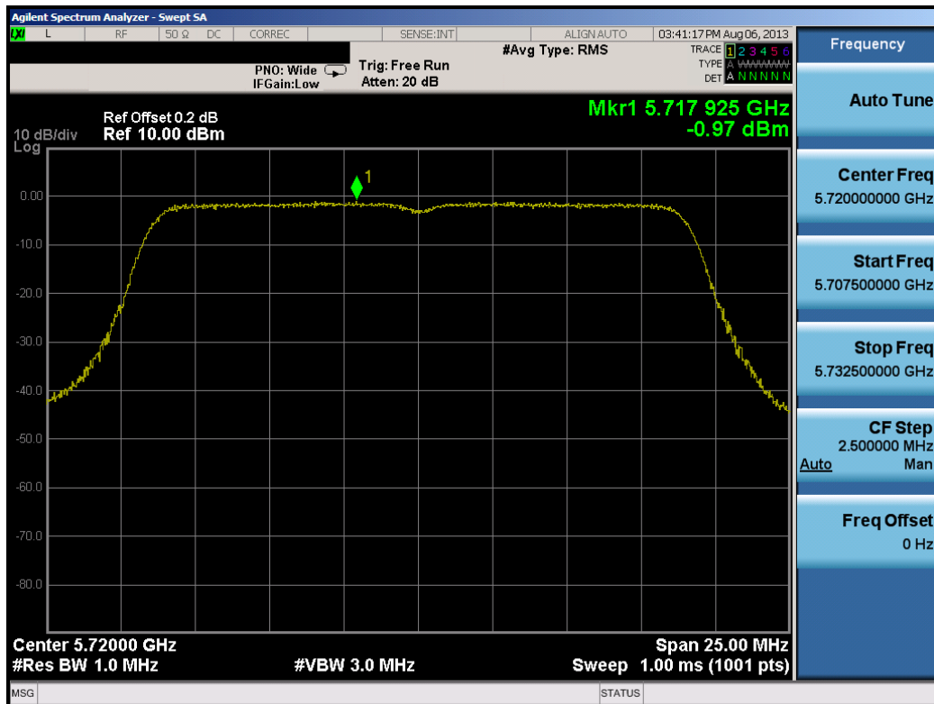
Plot 6-65. Peak Power Spectral Density Plot (20MHz BW 802.11n (UNII Band 3) – Ch. 144)
