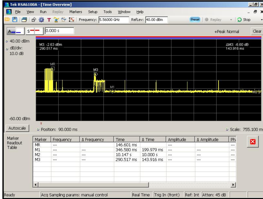
Figure 6-5. Move Time (zoomed in to around M1)
