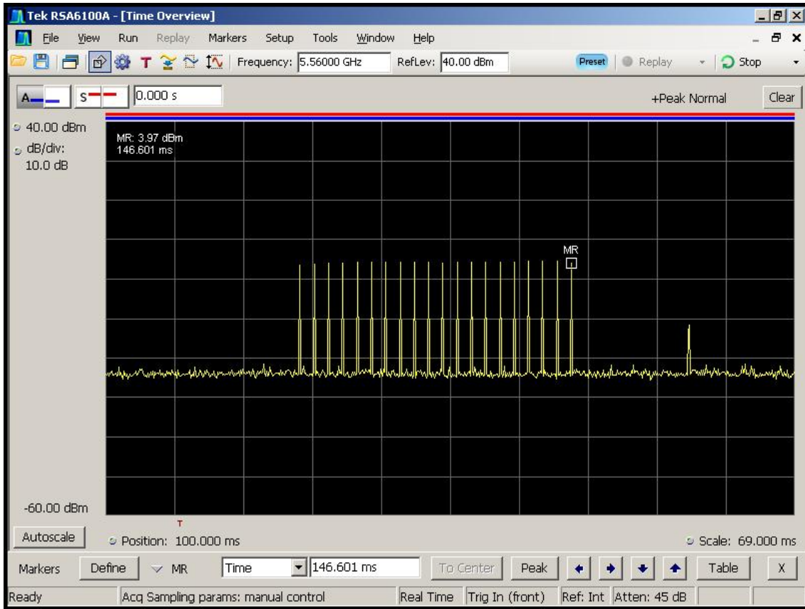
Figure 6-1. Type 1 Radar Pulse
