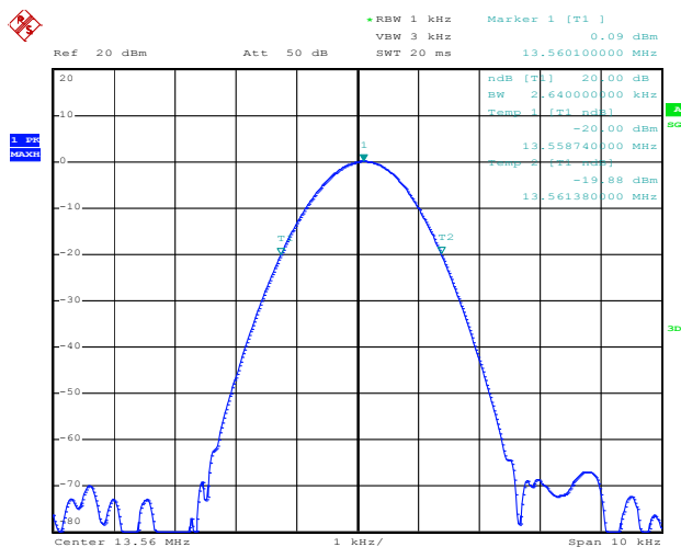
20 dB / 99% Bandwidth Plot on 13.56 MHz
