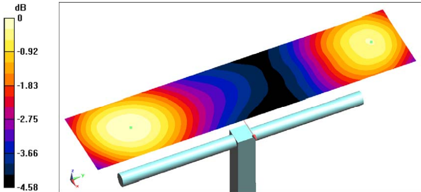
0 dB = 89.21 V/m = 39.01 dBV/m
