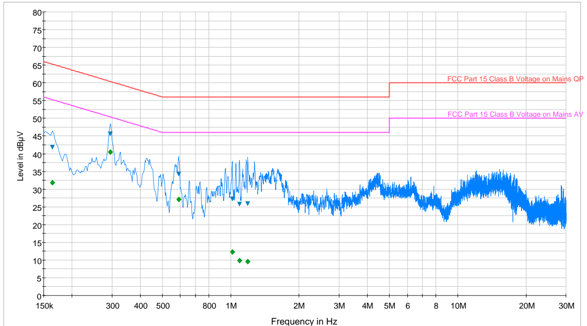
Plot 6-107. Line Conducted Plot with 802.11a UNII Band 3 (L1)
