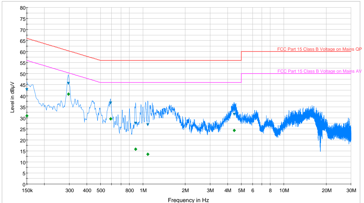
Plot 6-103. Line Conducted Plot with 802.11a UNII Band 1 (L1)
