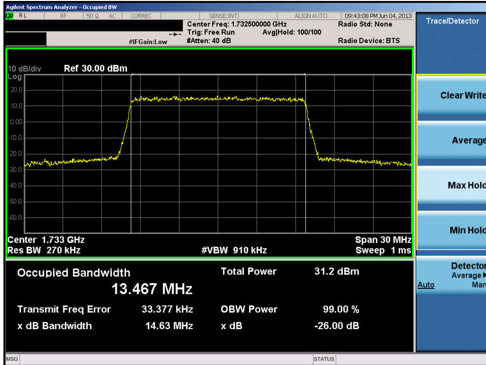
Plot 8-7. Occupied Bandwidth Plot (15.0MHz QPSK – RB Size 75)
