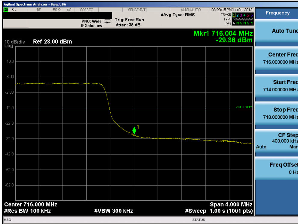
Plot 7-13. Upper Band Edge Plot (10.0MHz QPSK – RB Size 50)
