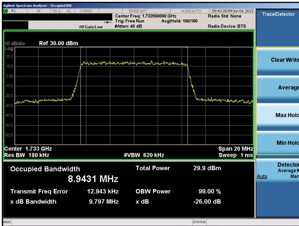
Plot 8-6. Occupied Bandwidth Plot (10.0MHz 16-QAM – RB Size 50)
