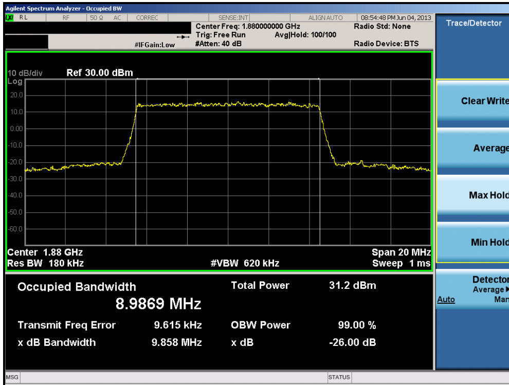
Plot 9-5. Occupied Bandwidth Plot (10.0MHz QPSK – RB Size 50)
