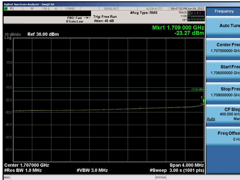
Plot 8-2. Lower Extended Band Edge Plot (10.0MHz QPSK – RB Size 50)
