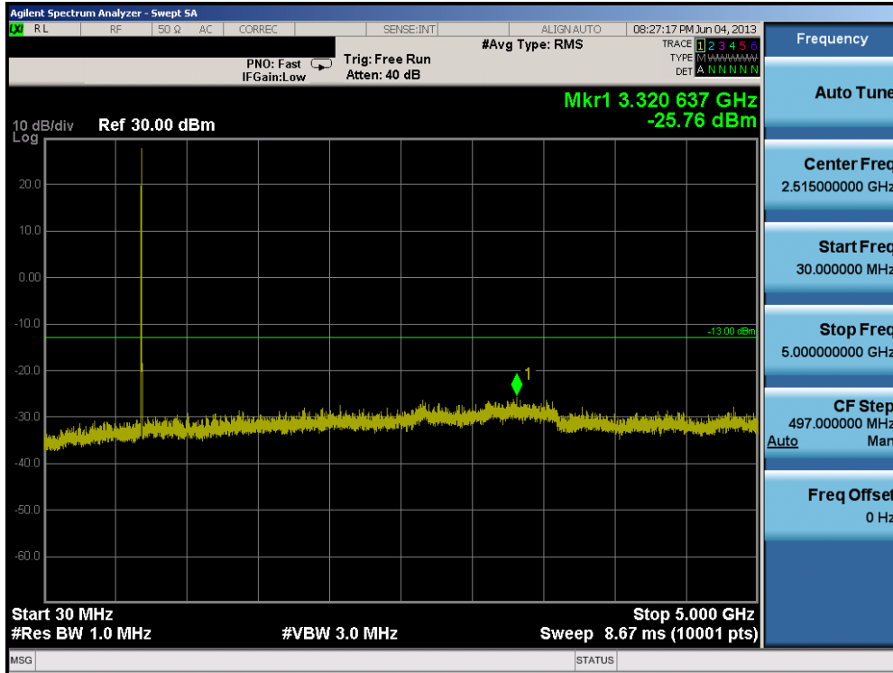
Plot 7-11. Conducted Spurious Plot (10.0MHz QPSK – RB Size 1, RB Offset 0 – High Channel)
