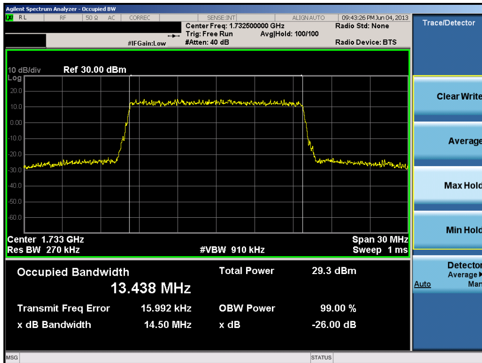
Plot 8-8. Occupied Bandwidth Plot (15.0MHz 16-QAM – RB Size 75)
