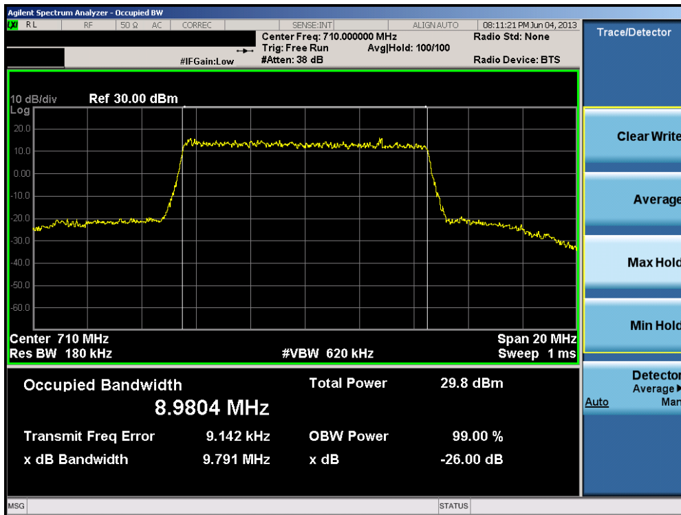
Plot 7-6. Occupied Bandwidth Plot (10.0MHz 16-QAM – RB Size 50)
