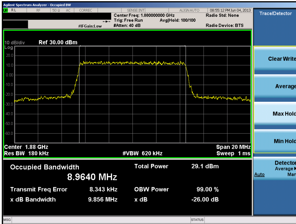
Plot 9-6. Occupied Bandwidth Plot (10.0MHz 16-QAM – RB Size 50)
