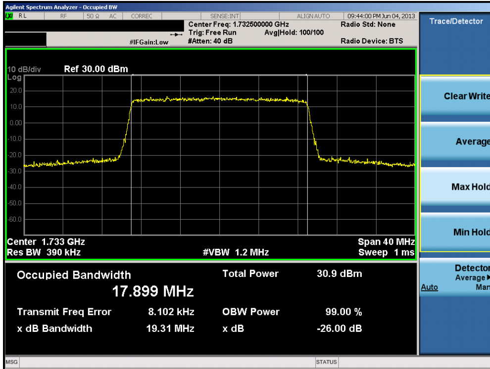
Plot 8-9. Occupied Bandwidth Plot (20.0MHz QPSK – RB Size 100)
