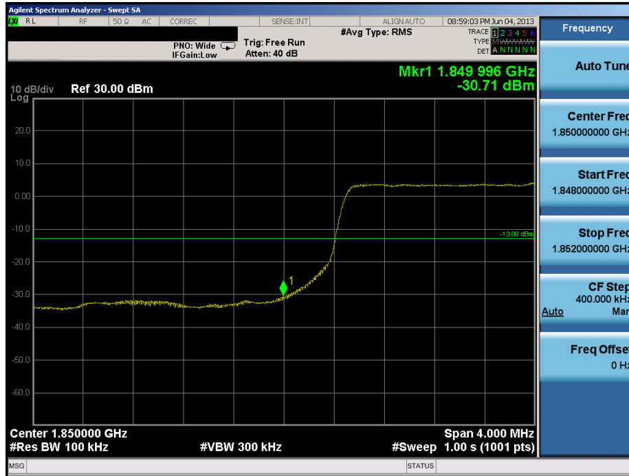
Plot 9-1. Lower Band Edge Plot (10.0MHz QPSK – RB Size 50)
