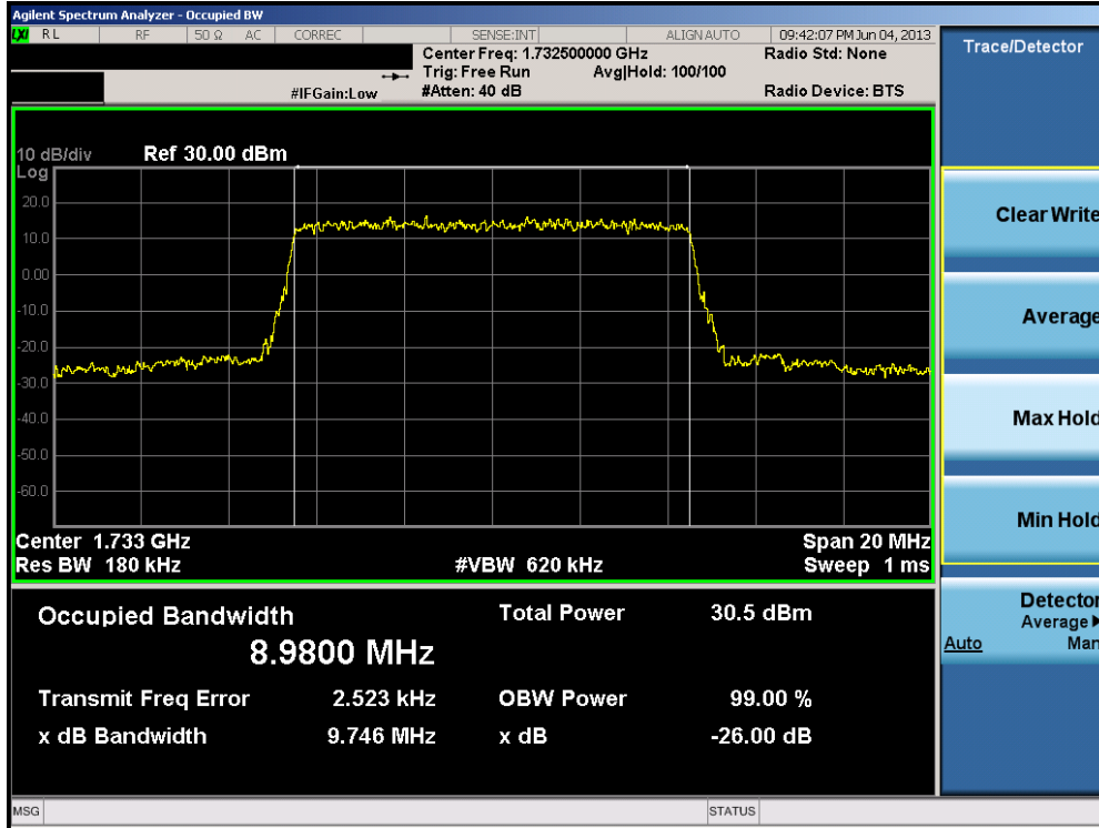
Plot 8-5. Occupied Bandwidth Plot (10.0MHz QPSK – RB Size 50)
