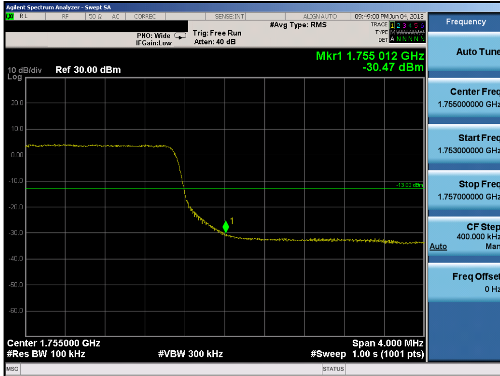
Plot 8-17. Upper Band Edge Plot (10.0MHz QPSK – RB Size 50)
