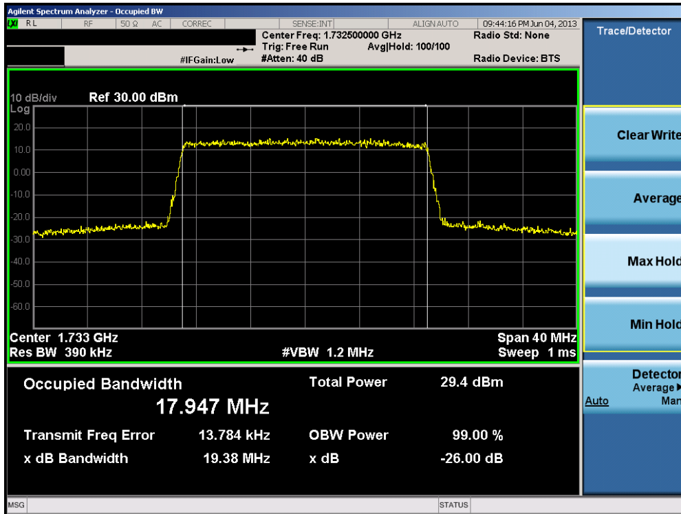
Plot 8-10. Occupied Bandwidth Plot (20.0MHz 16-QAM – RB Size 100)
