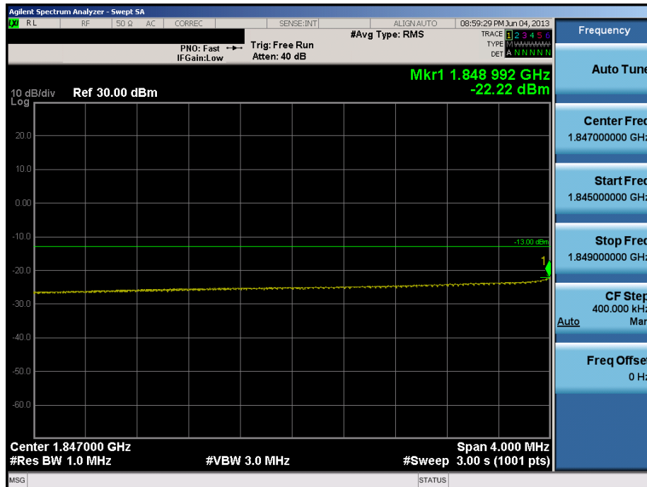
Plot 9-2. Lower Extended Band Edge Plot (10.0MHz QPSK – RB Size 50)
