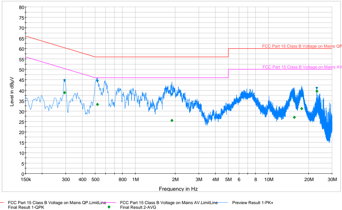
Plot 6-103. Line Conducted Plot with 802.11a UNII Band 2 (L1)
