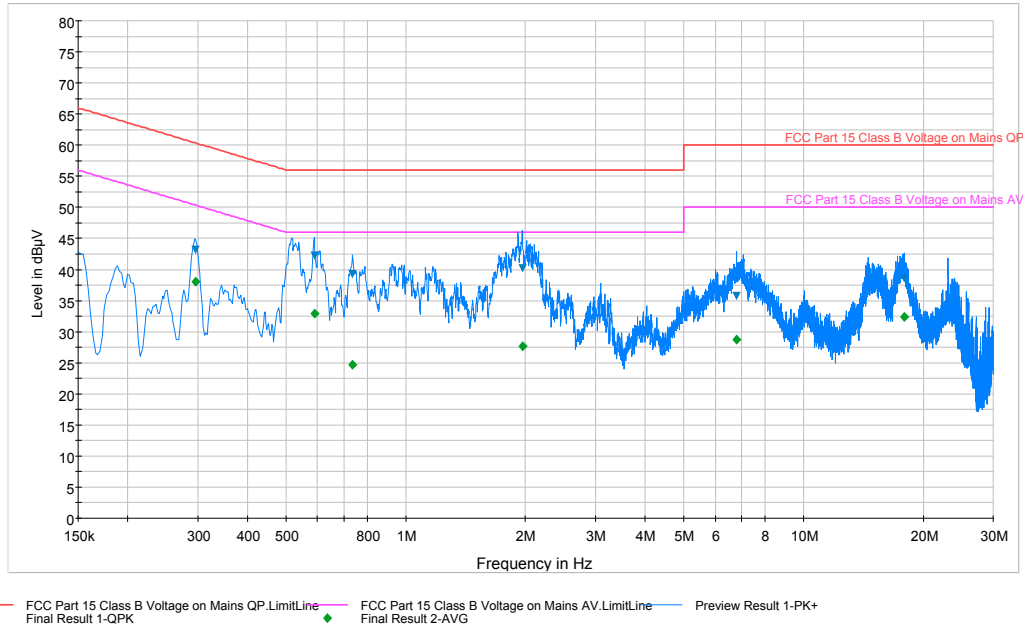
Plot 6-35. Line Conducted Plot with 802.11b (L1)
