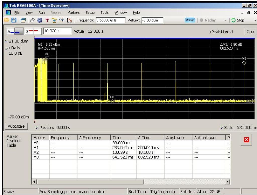
Figure 6-6. Aggregate Time Plot
