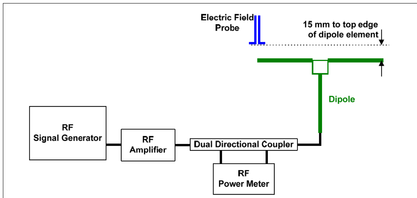
Setup diagram
