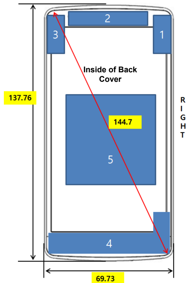
LG-D722J NFC Antenna Location
