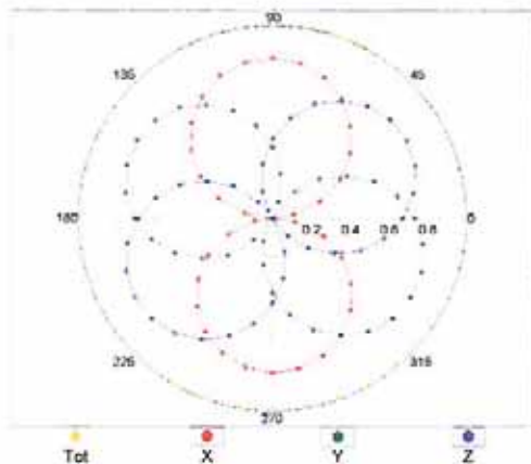
f=600 MHz,TEM
