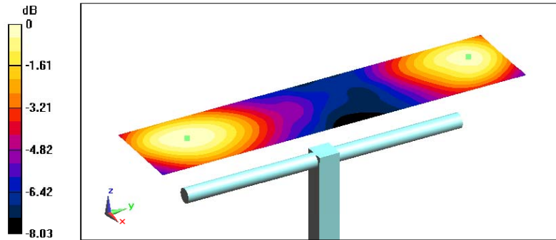
0 dB = 140.6V/m
