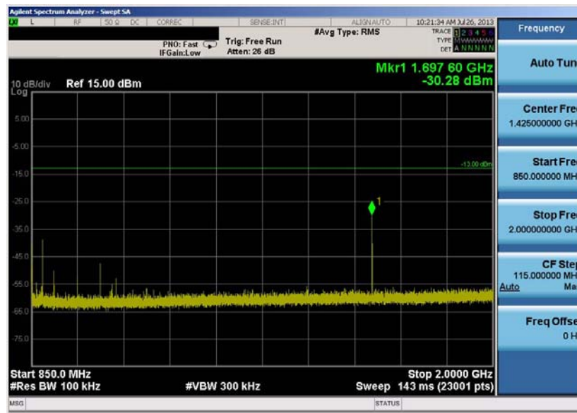
Plot 6-14. Conducted Spurious Plot (Cellular GSM Mode – Ch. 251)
