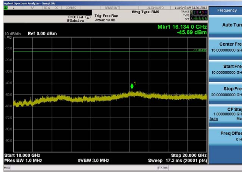
Plot 6-21. Conducted Spurious Plot (PCS GSM Mode – Ch. 810)
