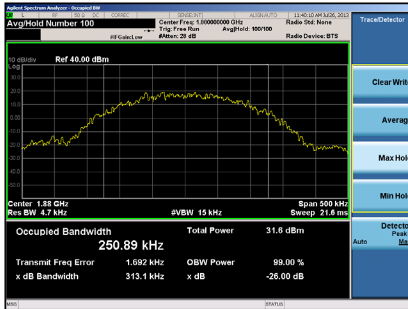
Plot 6-4. Occupied Bandwidth Plot (EDGE1900 Mode – Ch. 661)
