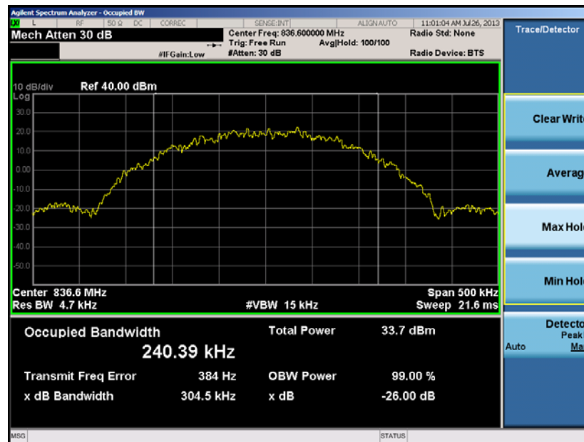
Plot 6-2. Occupied Bandwidth Plot (EDGE850 Mode – Ch. 190)
