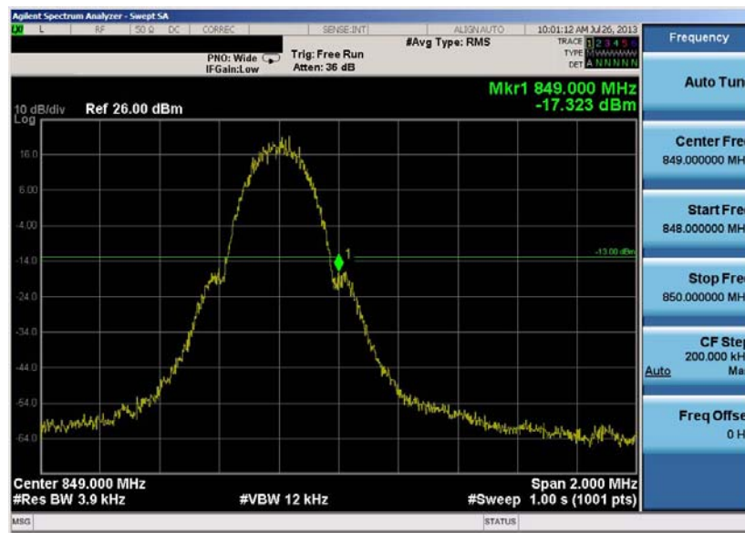
Plot 6-35. Band Edge Plot (Cellular GSM Mode – Ch. 251)
