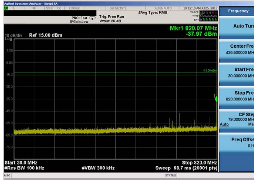
Plot 6-13. Conducted Spurious Plot (Cellular GSM Mode – Ch. 251)
