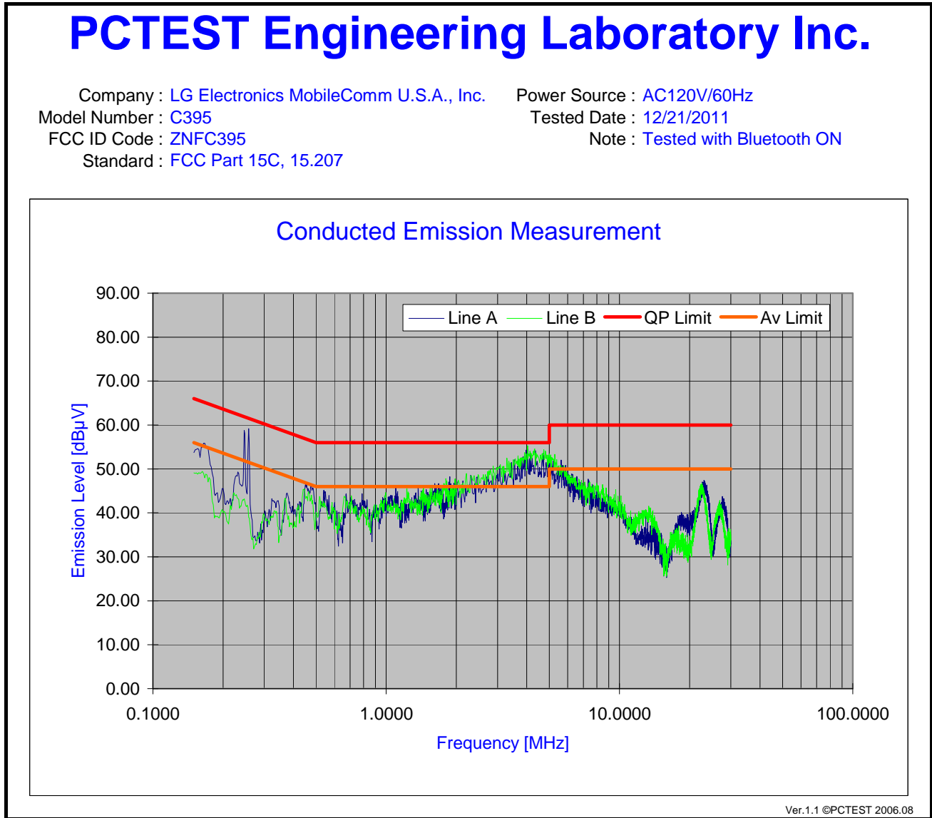
Plot 6-22. Line Conducted Plot with Bluetooth
