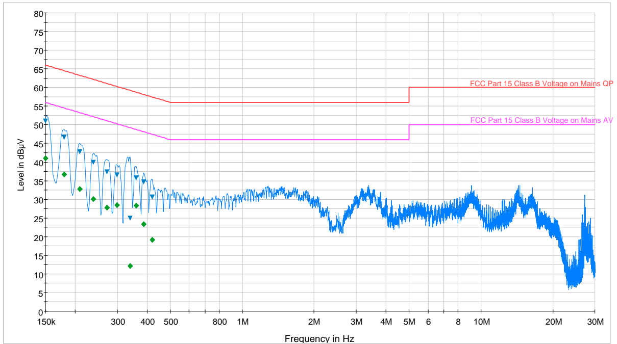
Plot 6-31. Line Conducted Plot with 802.11b (L1)
