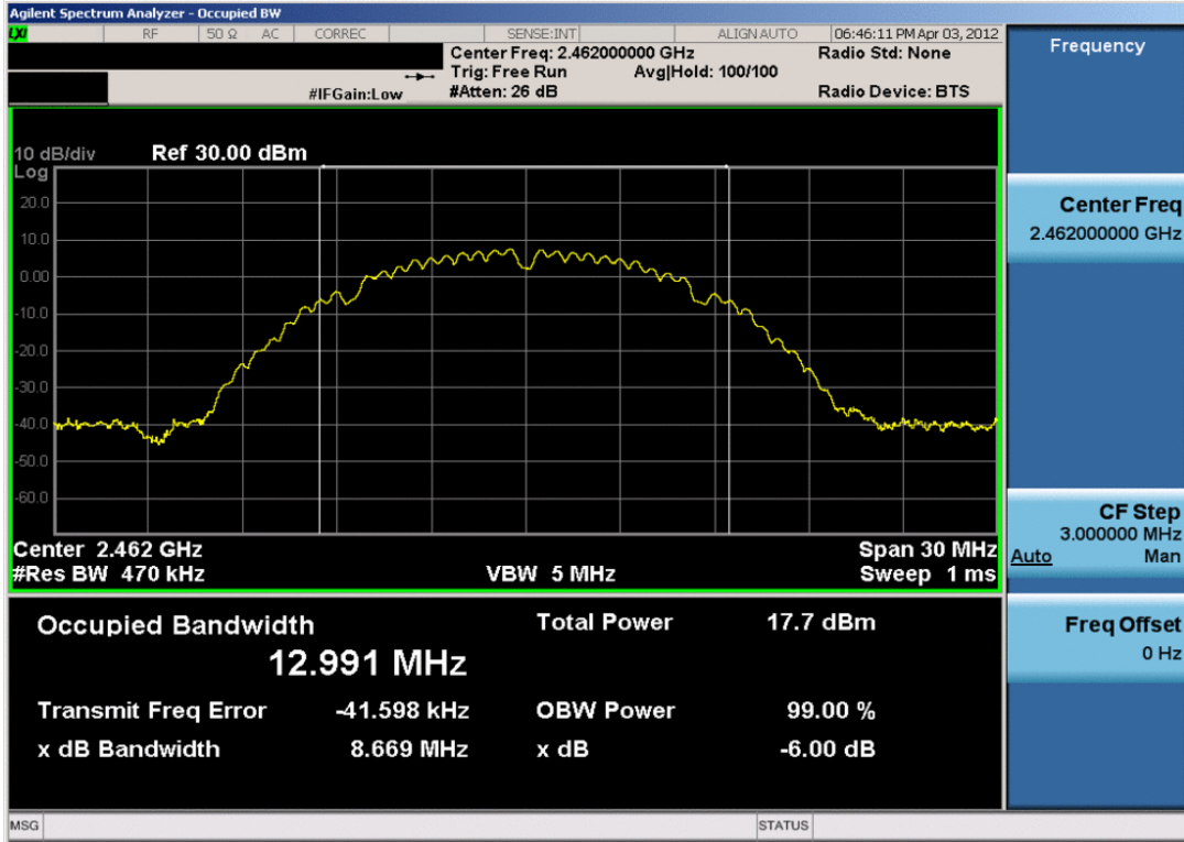
Plot 6-3. 6dB Bandwidth Plot (802.11b – Ch. 11)
