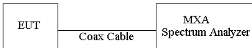
Figure 6-1. Test Instrument & Measurement Setup
