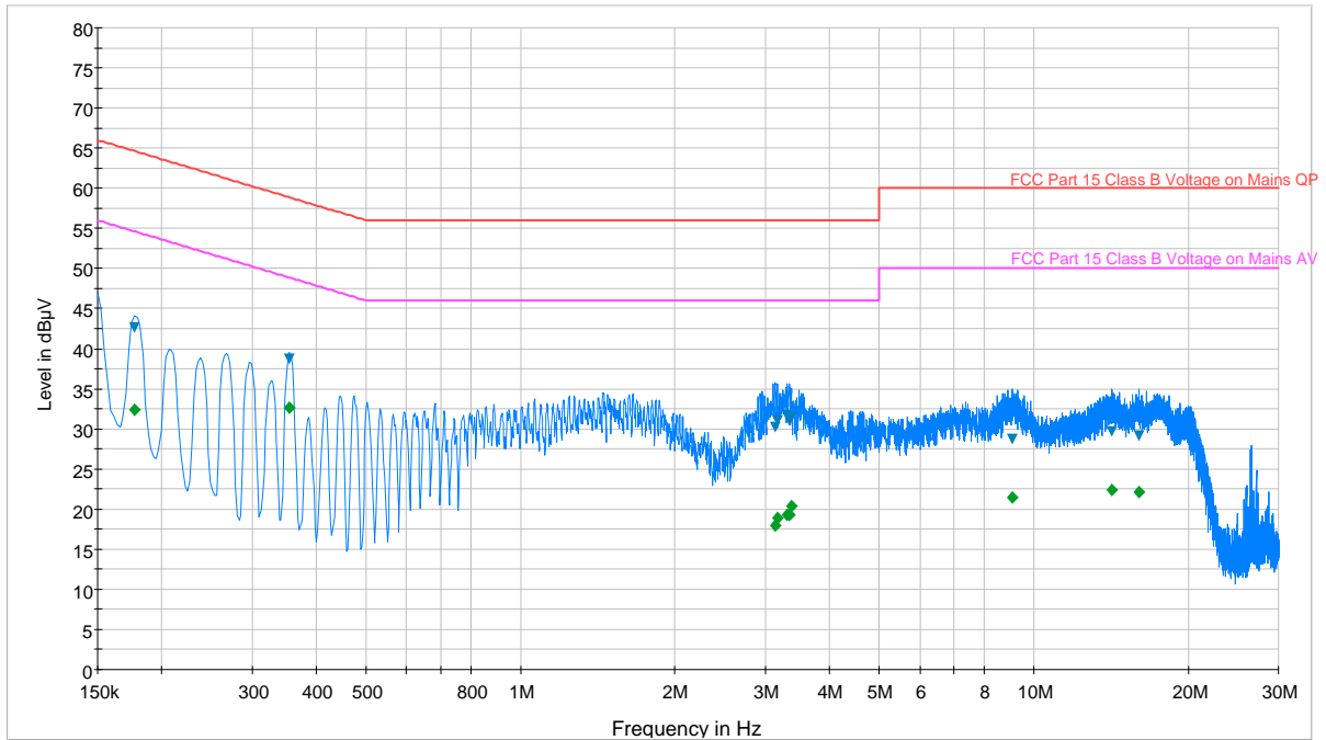
Plot 6-32. Line Conducted Plot with 802.11b (N)
