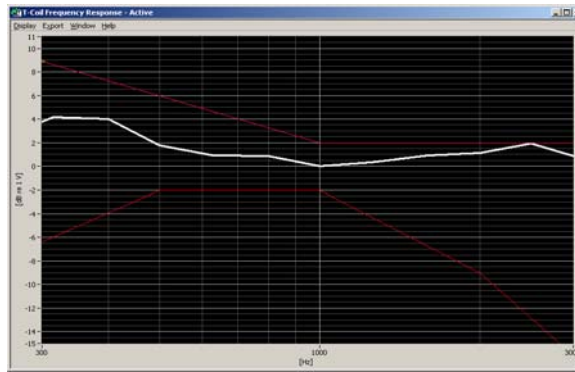
Figure 6-1 Axial Frequency Response
