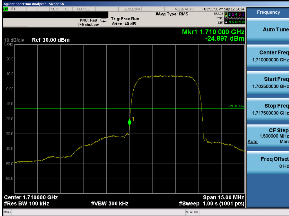
Plot 6-29. Band Edge Plot (AWS WCDMA Mode – Ch. 1312)
