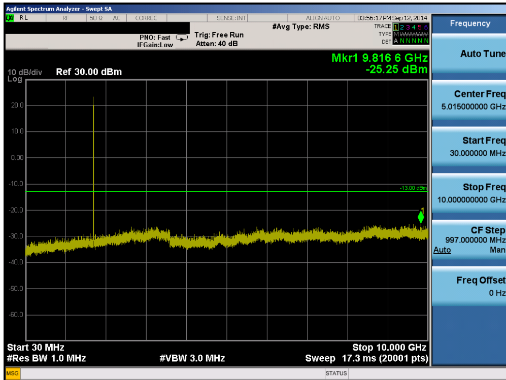
Plot 6-19. Conducted Spurious Plot (AWS WCDMA Mode – Ch. 1312)
