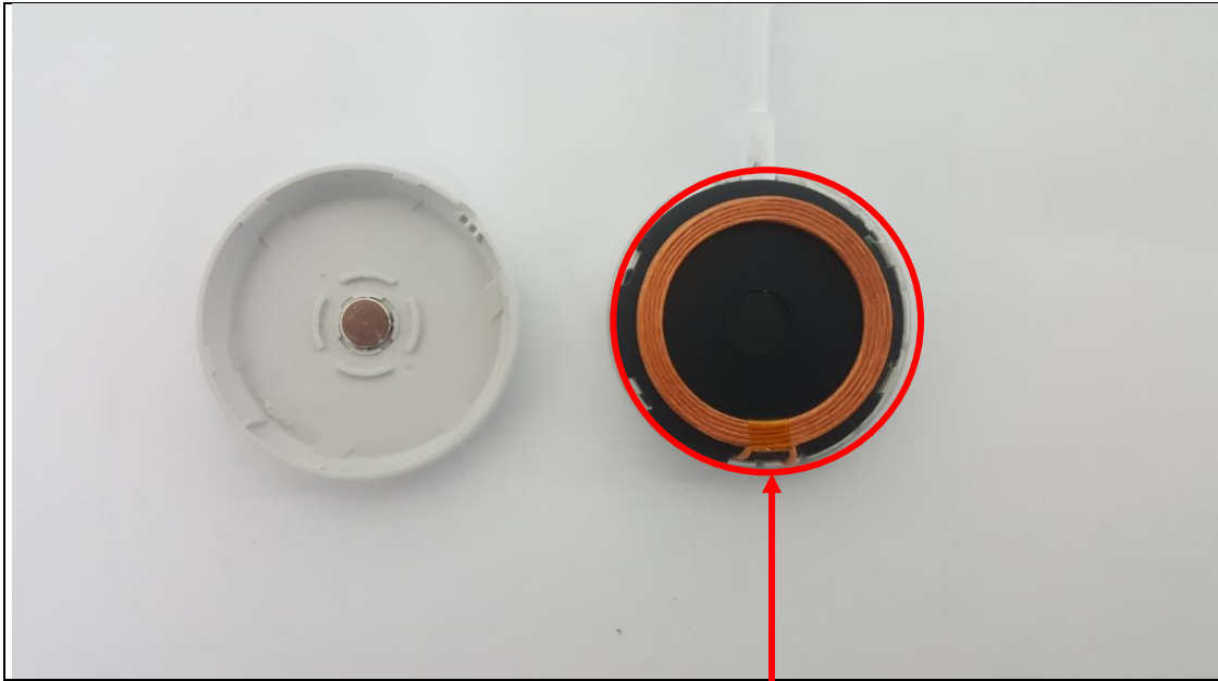
Inductive loop coil antenna
