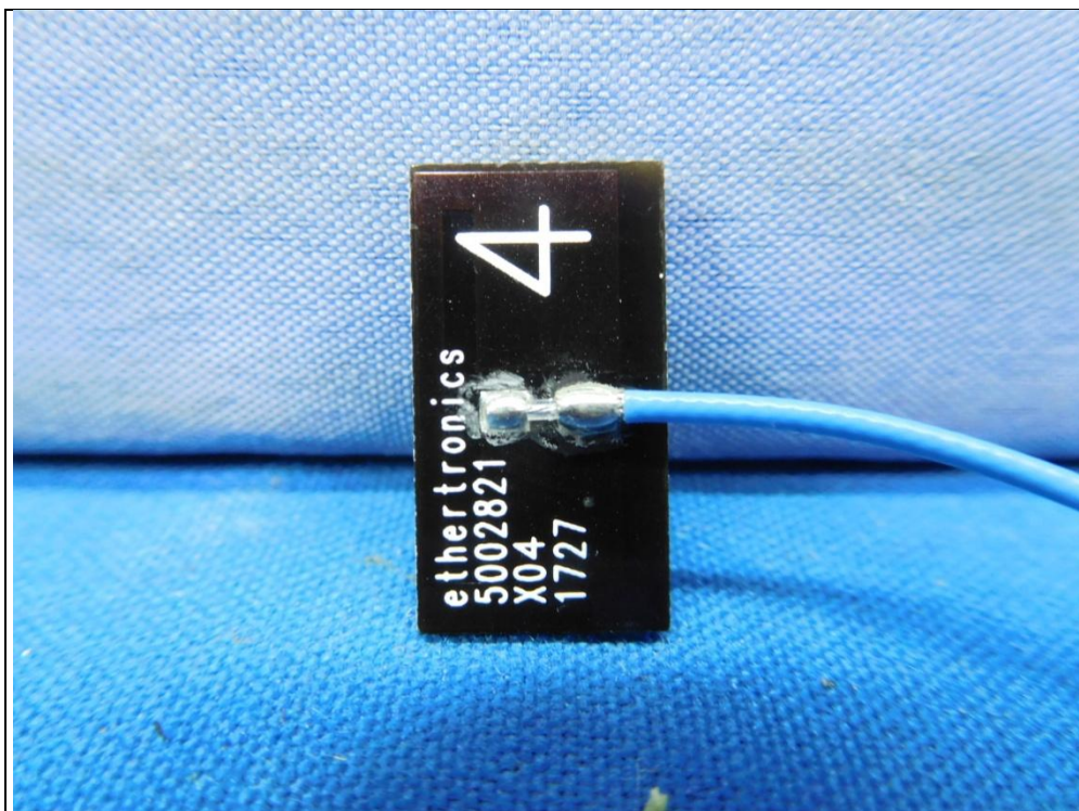
Antenna No.:5G1
