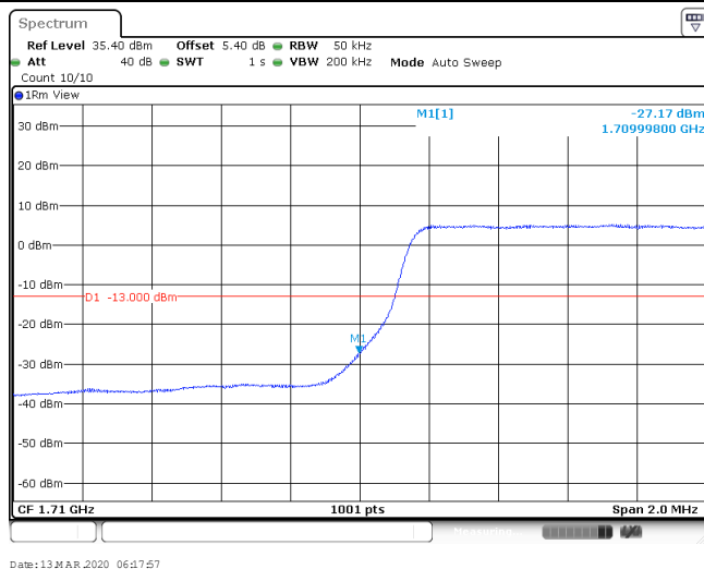
Band66_3MHz_16QAM_132657_1RB#14
