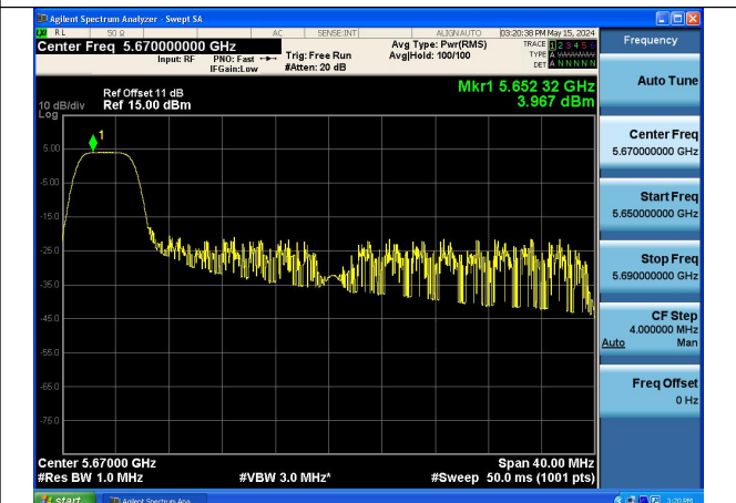
Mode:802.11ax HE40 Tone:52T Frequency:5670MHz Ant:Chain1
