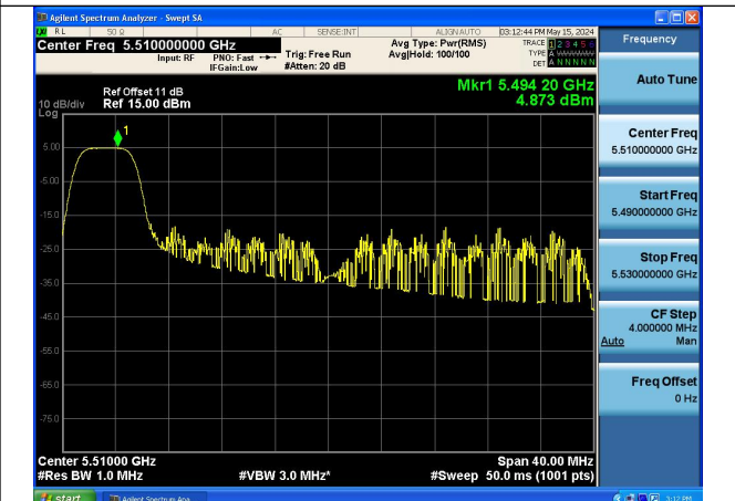
Mode:802.11ax HE40 Tone:52T Frequency:5510MHz Ant:Chain1
