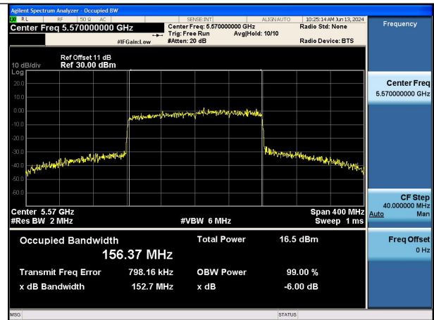
Mode:802.11ac VHT160 Frequency:5570MHz Ant:Chain1
