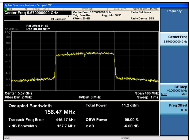
Mode:802.11ax HE160 Frequency:5570MHz Ant:Chain1
