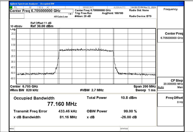
Mode:802.11ax HE80 Frequency:6705MHz Ant:Chain0
