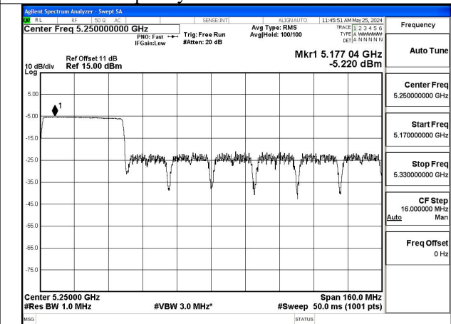
Mode:802.11ax HE160 Tone:484T Frequency:5250MHz Ant:Chain1
