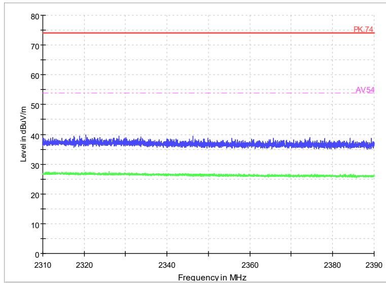
Radiated Emission Band Edge Channel No.:0 Test Mode: GFSK (LE 1Mbps) Polarization: H
