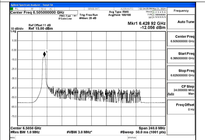
Mode:802.11ax HE160 Tone:52T Frequency:6505MHz Ant:Chain1
