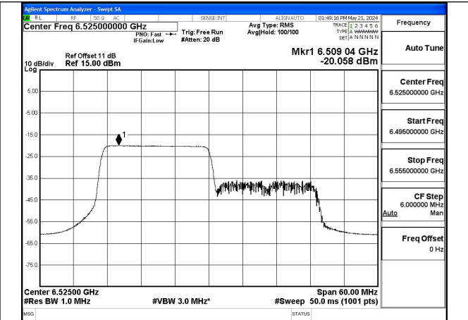
Mode:802.11ax HE40 Tone:242T Frequency:6525MHz Ant:Chain0
