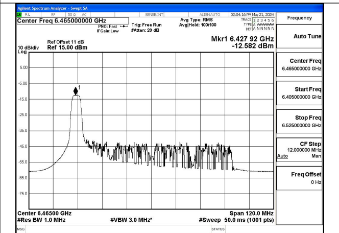
Mode:802.11ax HE80 Tone:52T Frequency:6465MHz Ant:Chain1
