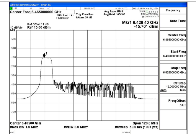
Mode:802.11ax HE80 Tone:106T Frequency:6465MHz Ant:Chain1
