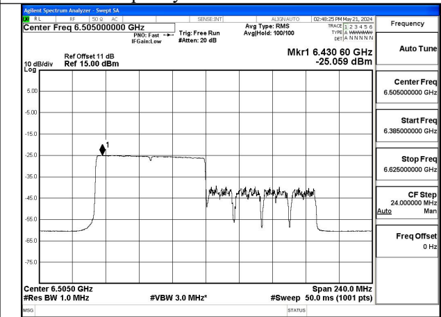
Mode:802.11ax HE160 Tone:996T Frequency:6505MHz Ant:Chain1
