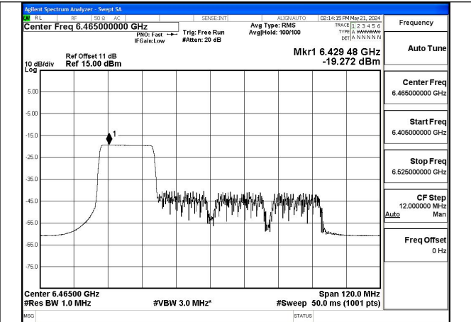
Mode:802.11ax HE80 Tone:242T Frequency:6465MHz Ant:Chain1
