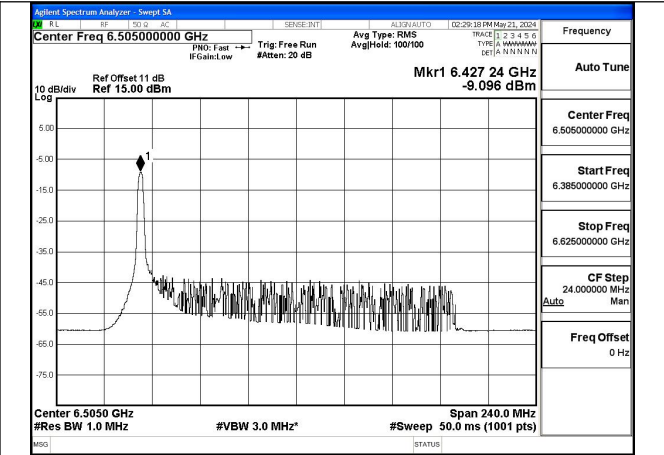
Mode:802.11ax HE160 Tone:26T Frequency:6505MHz Ant:Chain1
