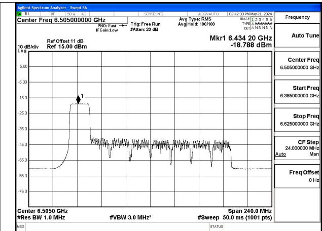
Mode:802.11ax HE160 Tone:242T Frequency:6505MHz Ant:Chain1
