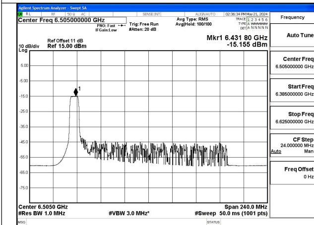
Mode:802.11ax HE160 Tone:106T Frequency:6505MHz Ant:Chain0
