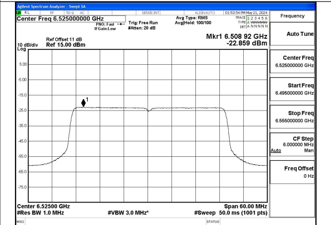
Mode:802.11ax HE40 Tone:484T Frequency:6525MHz Ant:Chain0
