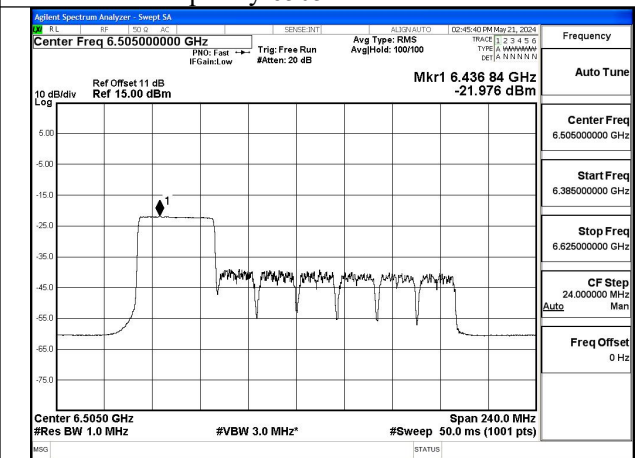
Mode:802.11ax HE160 Tone:484T Frequency:6505MHz Ant:Chain1
