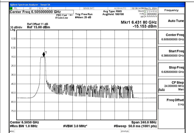
Mode:802.11ax HE160 Tone:106T Frequency:6505MHz Ant:Chain1
