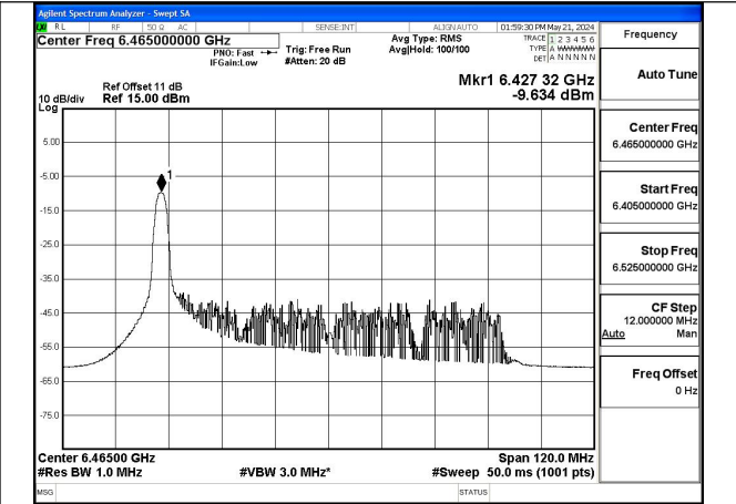
Mode:802.11ax HE80 Tone:26T Frequency:6465MHz Ant:Chain1
