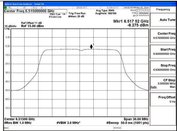
Mode:802.11a Frequency:6515MHz Ant:Chain1
