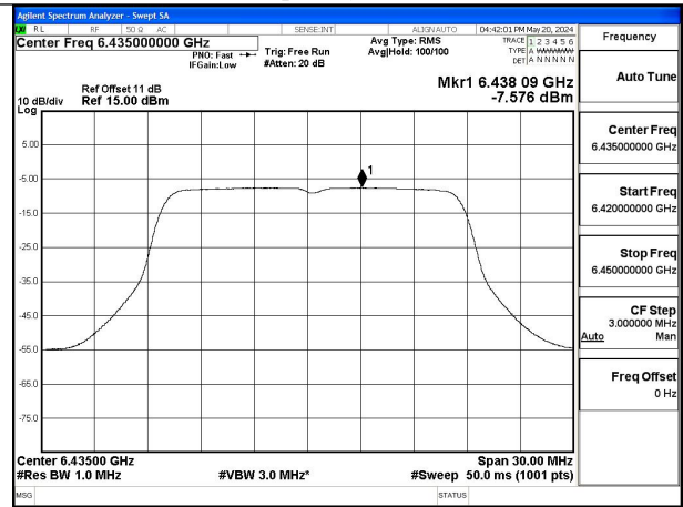
Mode:802.11a Frequency:6435MHz Ant:Chain1
