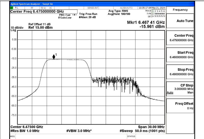
Mode:802.11ax HE20 Tone:106T Frequency:6475MHz Ant:Chain0
