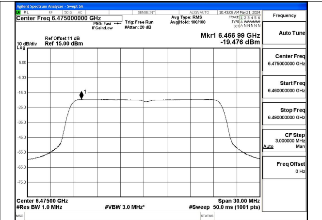
Mode:802.11ax HE20 Tone:242T Frequency:6475MHz Ant:Chain0
