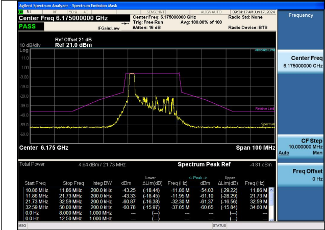
Mode:802.11ax HE20 Tone:26T Frequency:6175MHz Ant:Chain1
