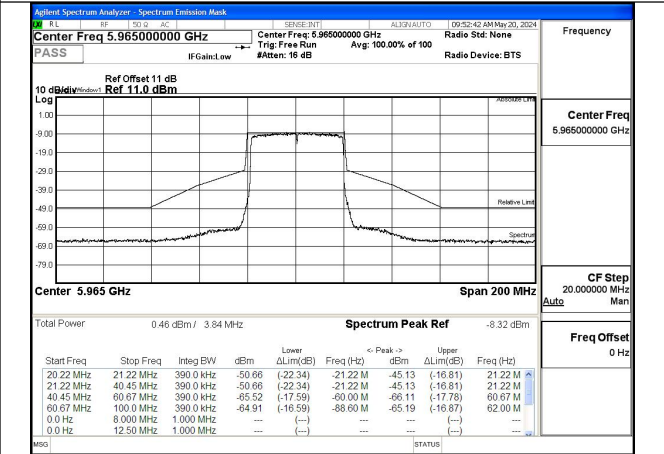
Mode:802.11ax HE40 Tone:242T Frequency:5965MHz Ant:Chain1
