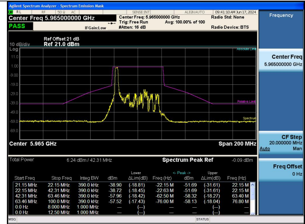
Mode:802.11ax HE40 Tone:26T Frequency:5965MHz Ant:Chain1
