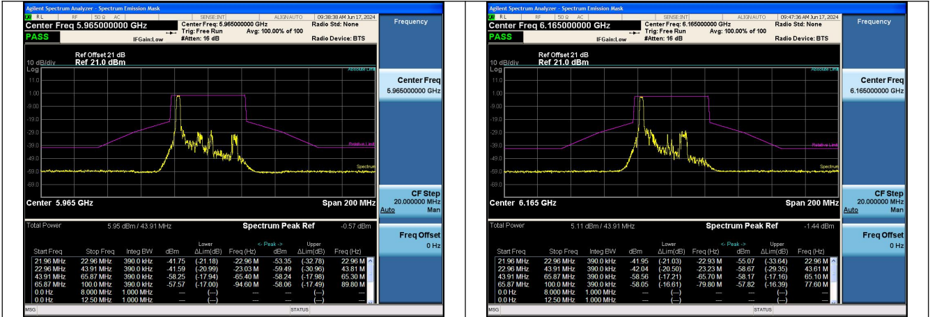
Mode:802.11ax HE40 Tone:26T Frequency:5965MHz Ant:Chain0
