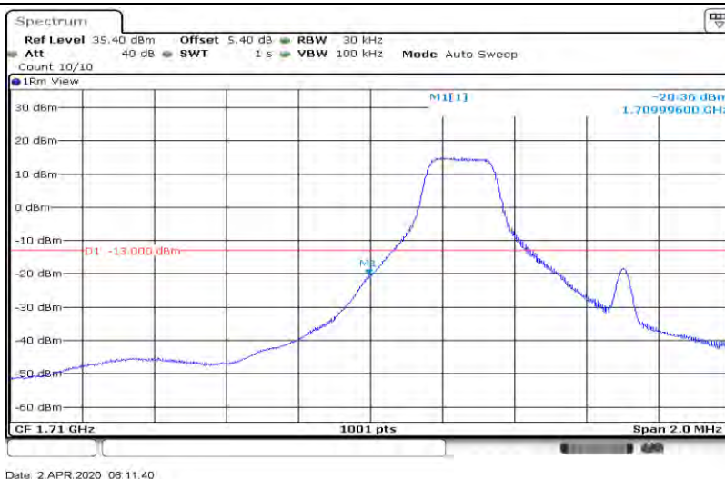
Band4-1.4MHz-16QAM-19957-6RB#0
