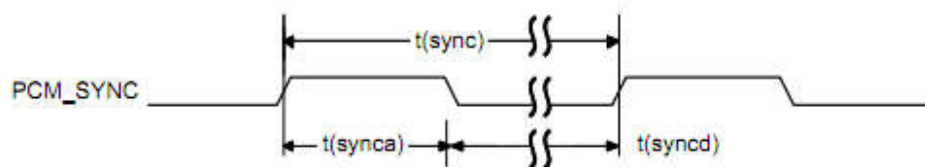
Figure 3-17 PCM_SYNC Timing
