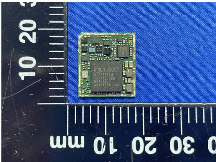
EUT UNCOVER VIEW (WITHOUT SHIELDING)
