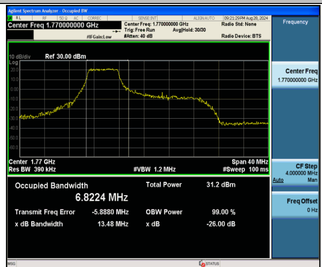
Band66-20MHz-16QAM-132572-27RB#0-PASS
