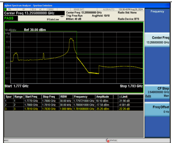
Band66-3MHz-QPSK-132657-1RB#14-PASS
