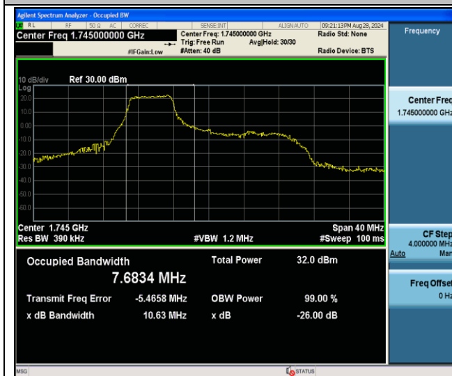
Band66-20MHz-16QAM-132322-27RB#0-PASS
