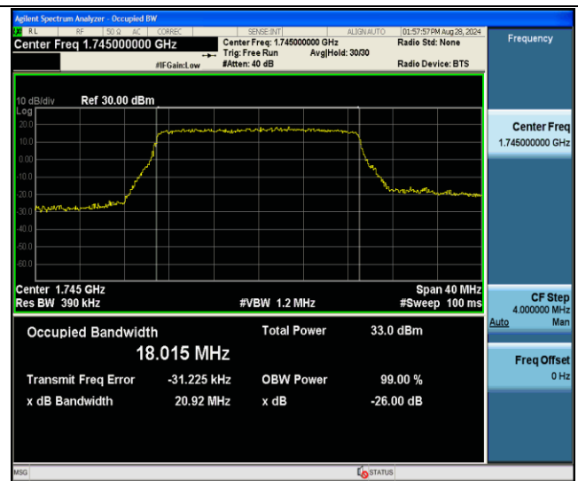
Band66-20MHz-QPSK-132322-100RB#0-PASS
