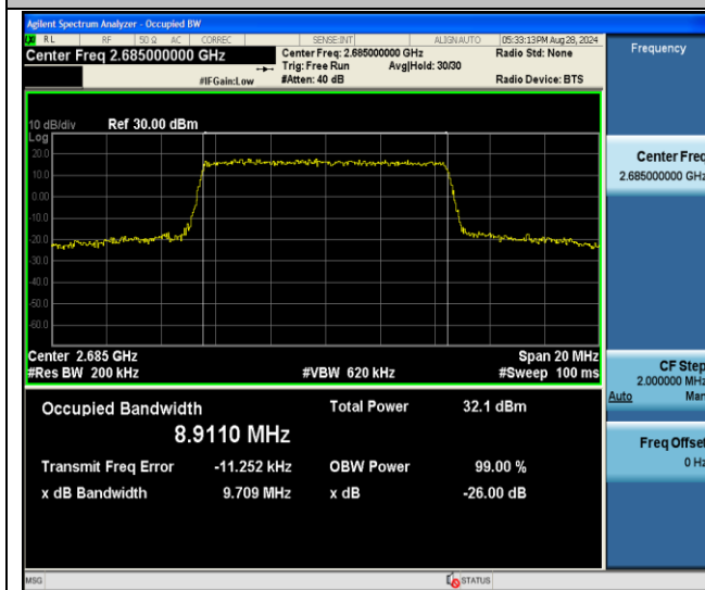
Band41-10MHz-QPSK-41540-50RB#0-PASS
