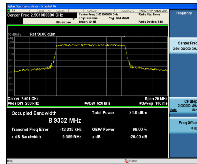
Band41-10MHz-QPSK-39700-50RB#0-PASS
