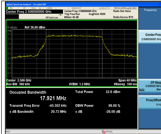
Band41-20MHz-QPSK-39750-100RB#0-PASS
