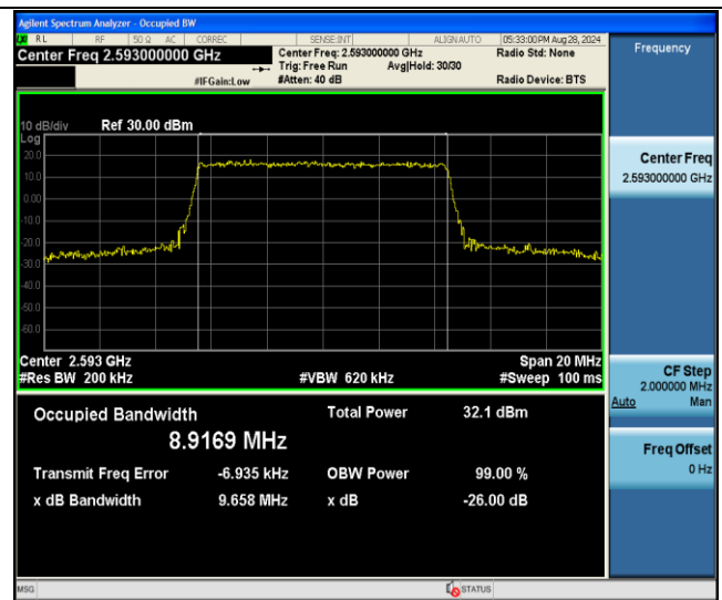
Band41-10MHz-QPSK-40620-50RB#0-PASS
