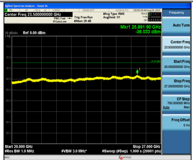
Band7-20MHz-QPSK-21350-1RB#0-20000~27000-PASS
