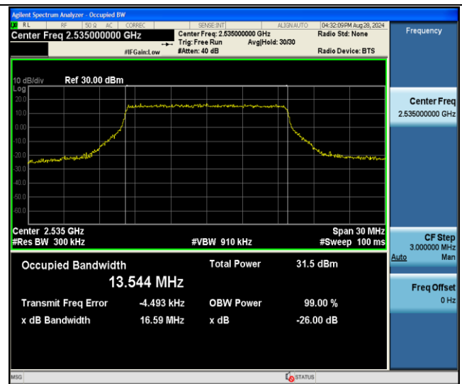
Band7-15MHz-QPSK-21100-75RB#0-PASS
