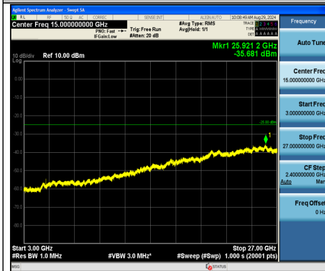
Band7-20MHz-QPSK-21350-1RB#0-3000~27000-PASS
