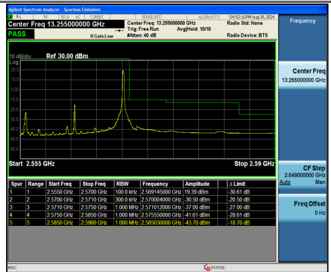
Band7-15MHz-QPSK-21375-1RB#74-PASS
