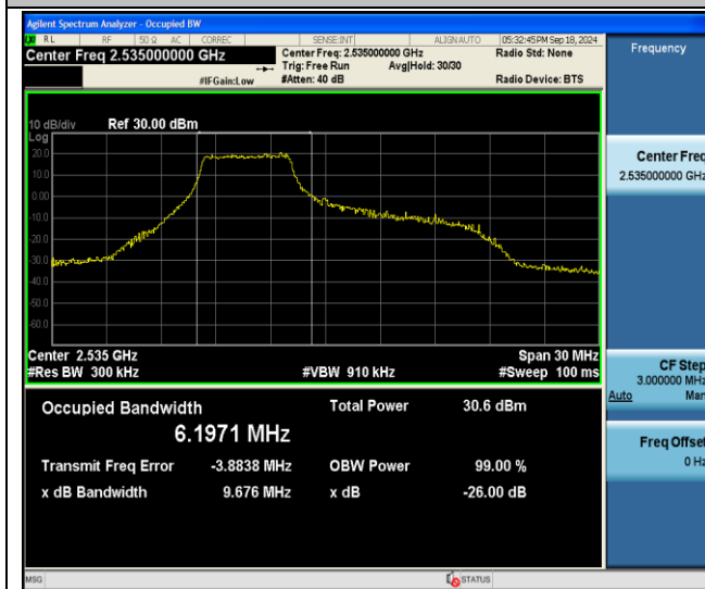
Band7-15MHz-16QAM-21100-27RB#0-PASS
