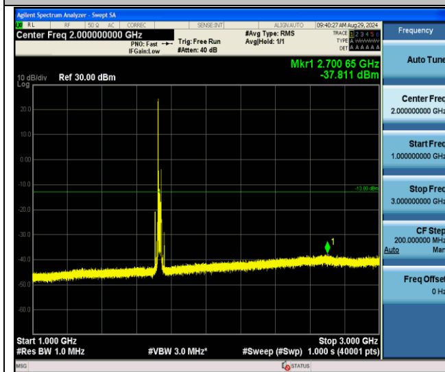
Band4-20MHz-QPSK-20175-1RB#0-1000~3000-PASS
