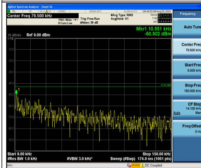
Band4-20MHz-QPSK-20300-1RB#0-0.009~0.15-PASS
