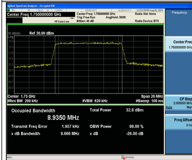
Band4-10MHz-QPSK-20350-50RB#0-PASS
